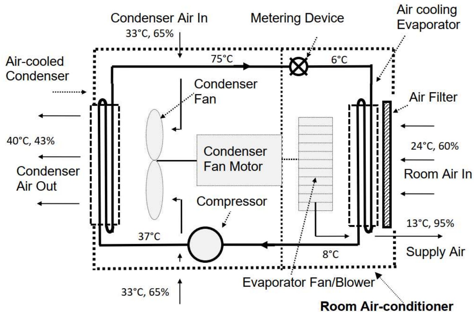
Figure 1.5 – Room Air-conditioner Schematic
